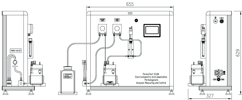
Fig. 1 - Instrumentation panel
