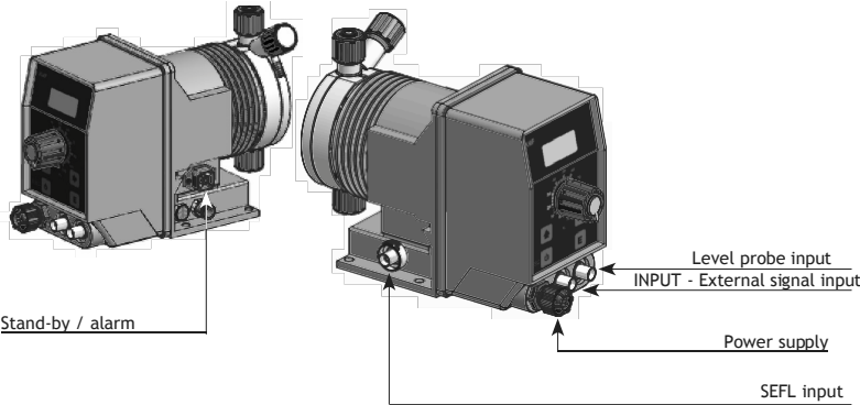
Fig. 12. Pump connections
