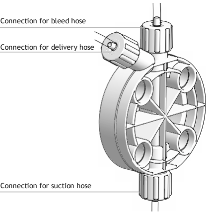
Fig. 8. Description of the self-purging pump body (KMSA MF pump)
