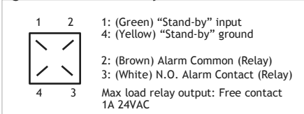
Fig. 11. Alarm/stand-by connection
