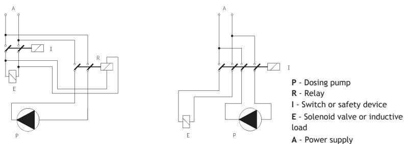
Fig. 10. Electrical installation of the pump
