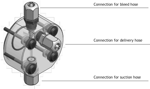
Fig. 9. Description of the self-purging pump body in PMMA (KMSA MF pump)
