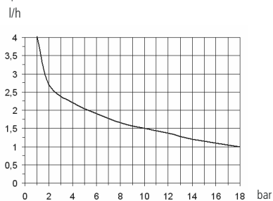
1801: l/h 1 bar 18 Pump head mod. LA
