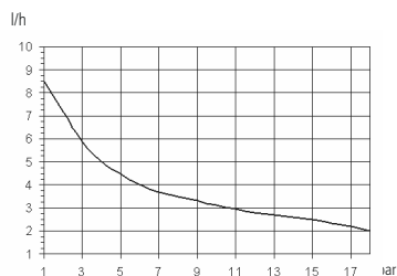
1005: l/h 5 bar 10 Pump head mod. L
