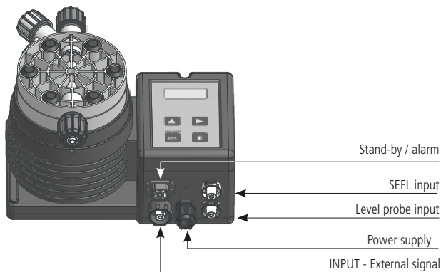
Fig. 15. Pump's connections
