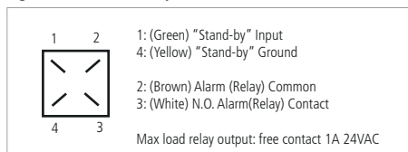
Fig. 14. Alarm/stand-by connection
