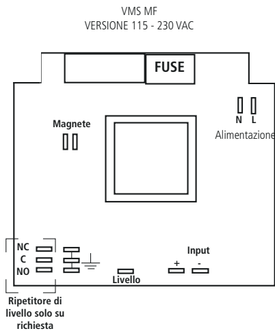
Fig. 38. Schema circuito VMS MF / VMSA MF
