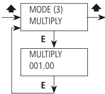
Fig. 16. Menù Multiply.
