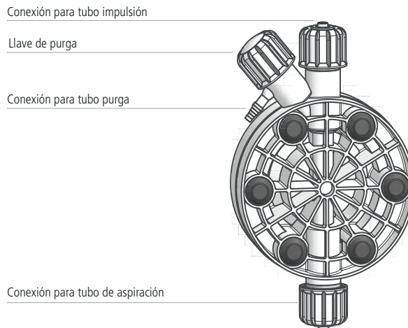
Fig. 5. Cabezal purga manual (T).
