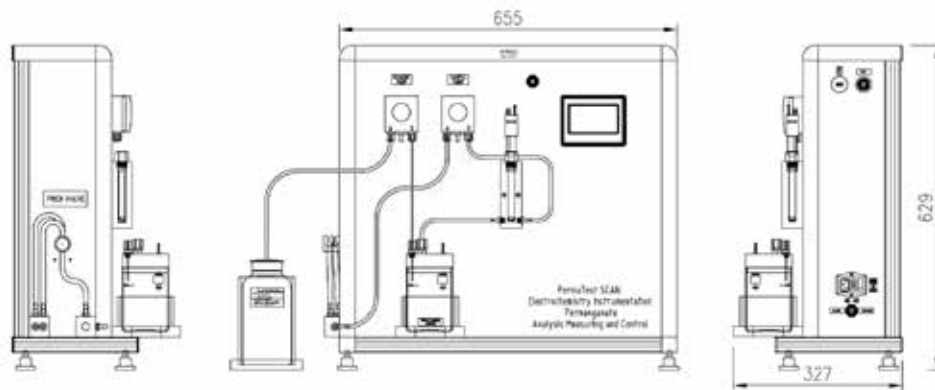
Fig. 1 - Instrumentation panel
